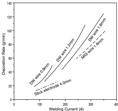
Fig. 1 Deposition rate as per welding current
