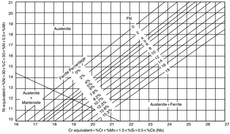
Fig. 2 DeLong Diagram
